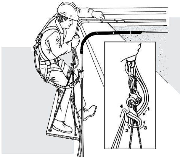
Figure 8 Bosun's Chair with Descent Control Device
