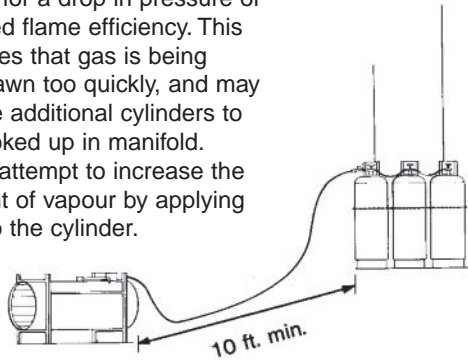
Typical Manifold Set-Up Figure 7
