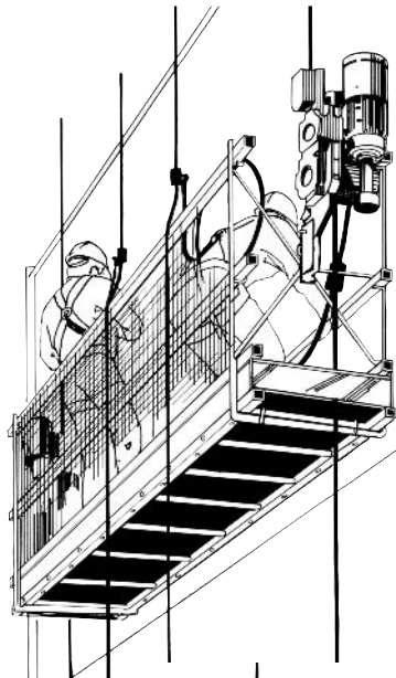
Figure 5 Powered Drum Hoist Climber Equipped Stage
