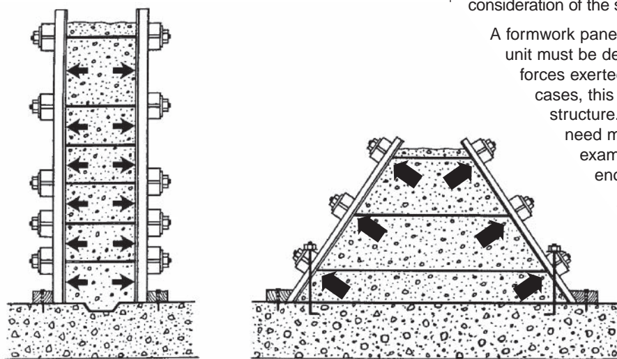
Figure 190 — Pressure of Concrete on Vertical and Battered Formwork (Note expansion anchors holding down battered form.)
