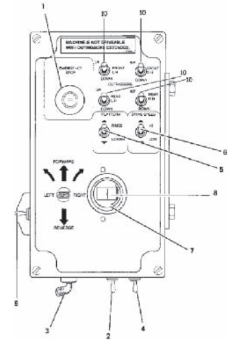
Figure 1.2: Example of controls on scissor-type platforms
