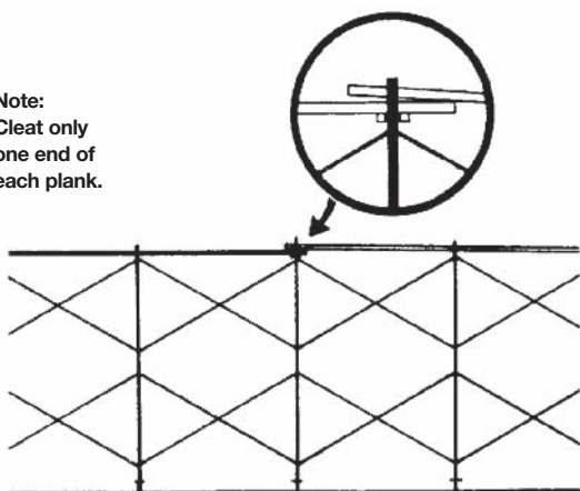
Figure 8.5 OVERLAPPING PLANKS FOR MULTI-SPAN TOWERS
