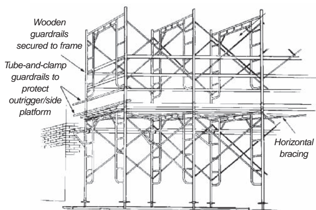
Figure 4.2 WALK-THROUGH SCAFFOLD
