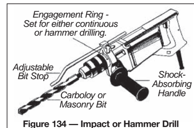
Figure 134 — Impact or Hammer Drill
