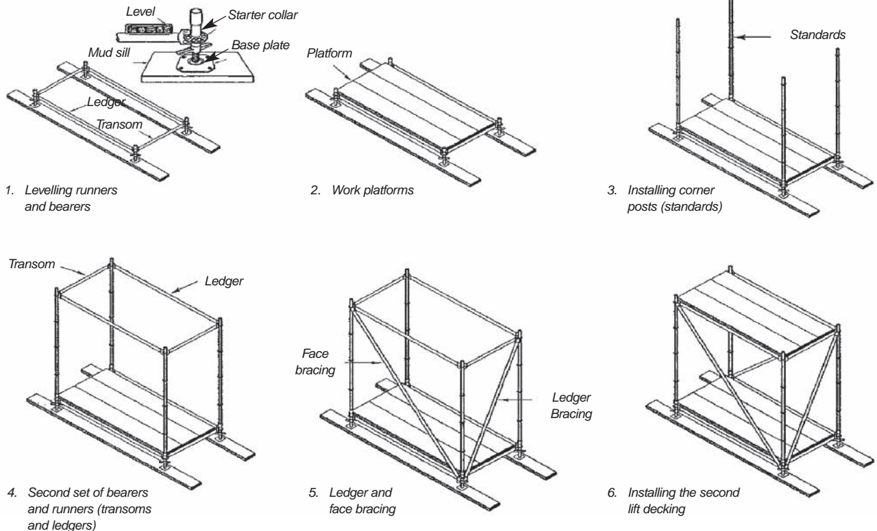
Figure 6.10 ERECTION SEQUENCE OF TYPICAL SYSTEMS SCAFFOLD
