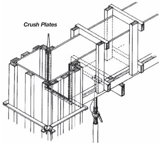
Figure 192 – Crush Plates
