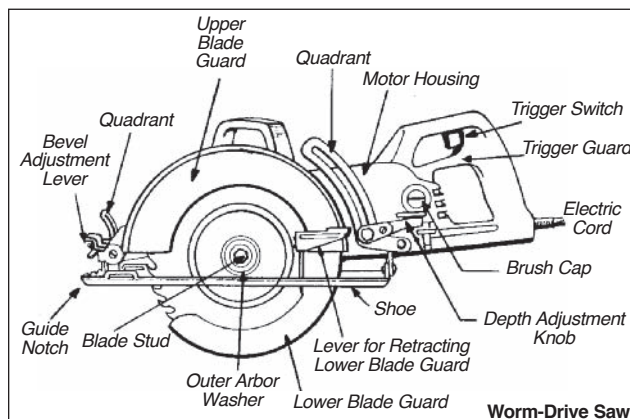
Worm-Drive Saw
