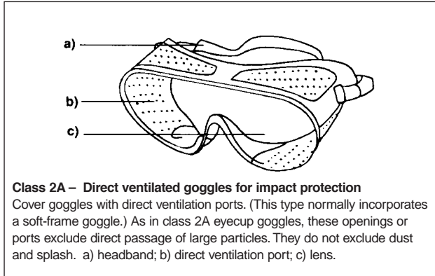
Figure 5 – Cover Goggles
