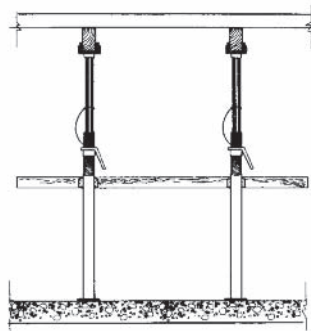
Figure 209 Single-Post Shores with Lateral Bracing
