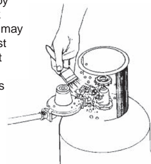
Figure 6 - Soap Test for Leaks
