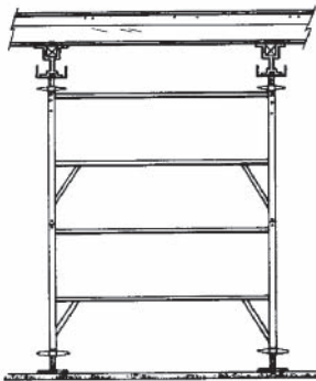
Figure 207 Typical Shoring Tower with Stringers, Adjustable Base Plates, and U-Heads
