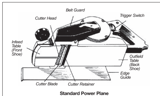
Standard Power Plane
