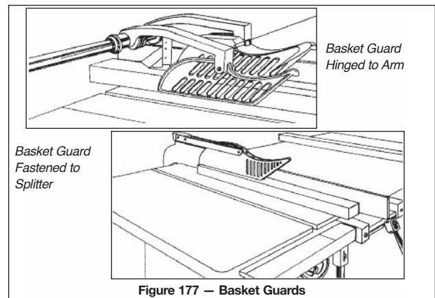
Figure 177 – Basket Guards
