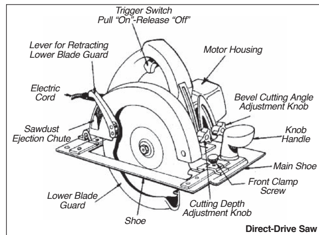
Direct-Drive Saw
