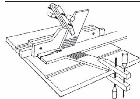
Figure 184 — Feather Boards
