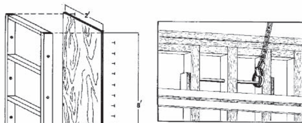
Figure 192 – Crush Plates
