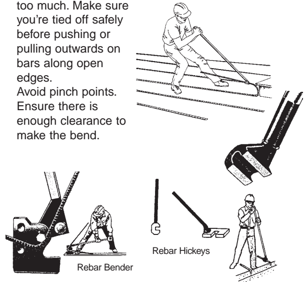
Figure 1.9: Hand Benders
