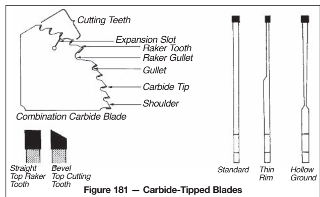
Figure 181 — Carbide-Tipped Blades
