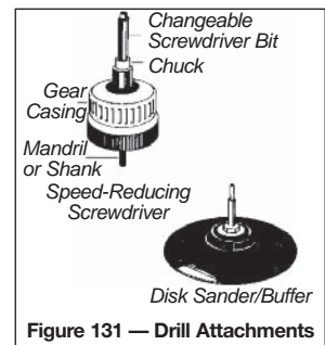
Figure 131 — Drill Attachments
