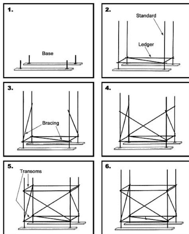
Figure 6.6 ERECTON OF TUBE-AND-CLAMP SCAFFOLD
